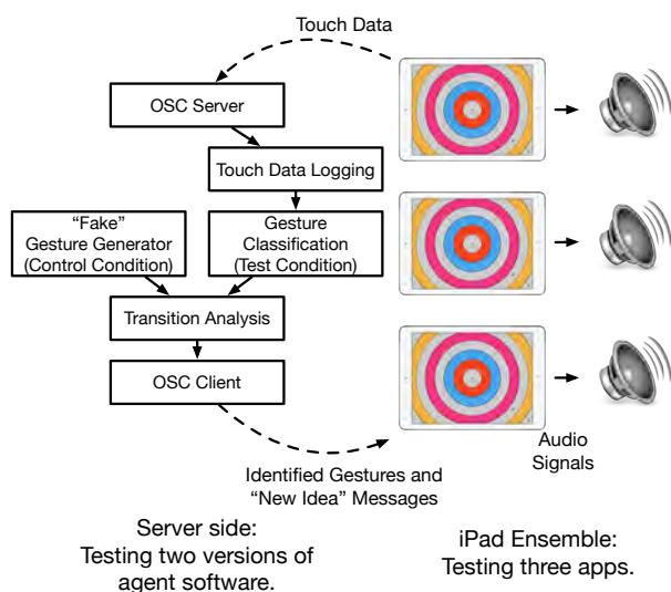
Figure 1. A system diagram of our agent software interacting with our iPad instruments. In the test condition, touch messages are classified as gestures by a Random Forest classifier, while in the control, gestures are generated from a statistical model disconnected from the performers’ current actions.
